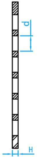
CROSS SECTIONAL VIEW
